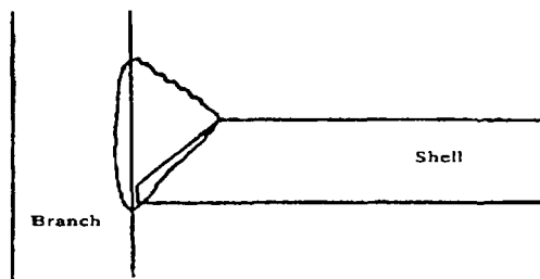
Figure 6.12 d : Partial penetration "set through" weld.
