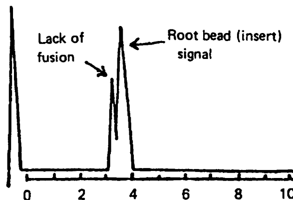
Figure 6.25 : CRT indication for lack of fusion at root.
