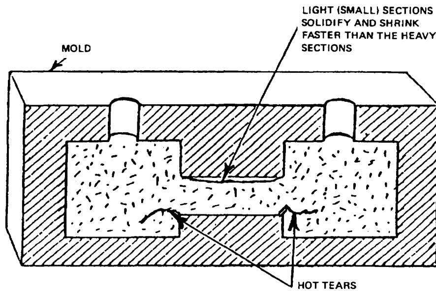
Figure 1.23 : Hot tears.
