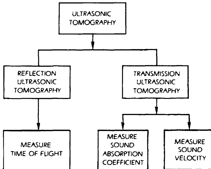
Figure 9.8 : Parameters determined in ultrasonic tomography.
