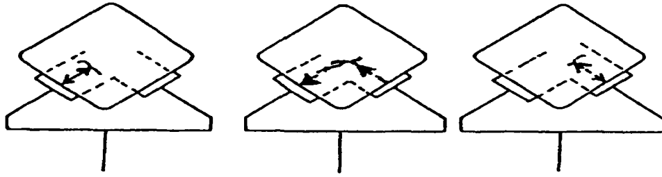
Figure 6.48 : Testing billets with two probes connected in parallel.
