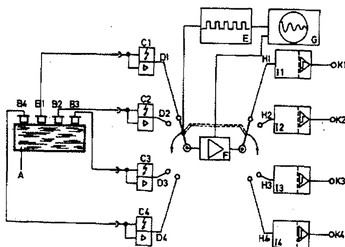
Figure 4.8 : Schematic diagram of a four channel flaw detection system.
