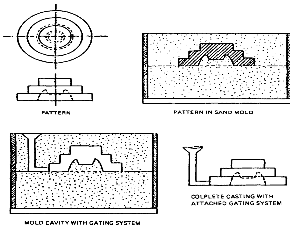
Figure 1.17 : Casting steps.
