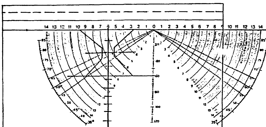
Figure 8.12 : Location of defect as described in 8.1.4.3.2 (vi).
