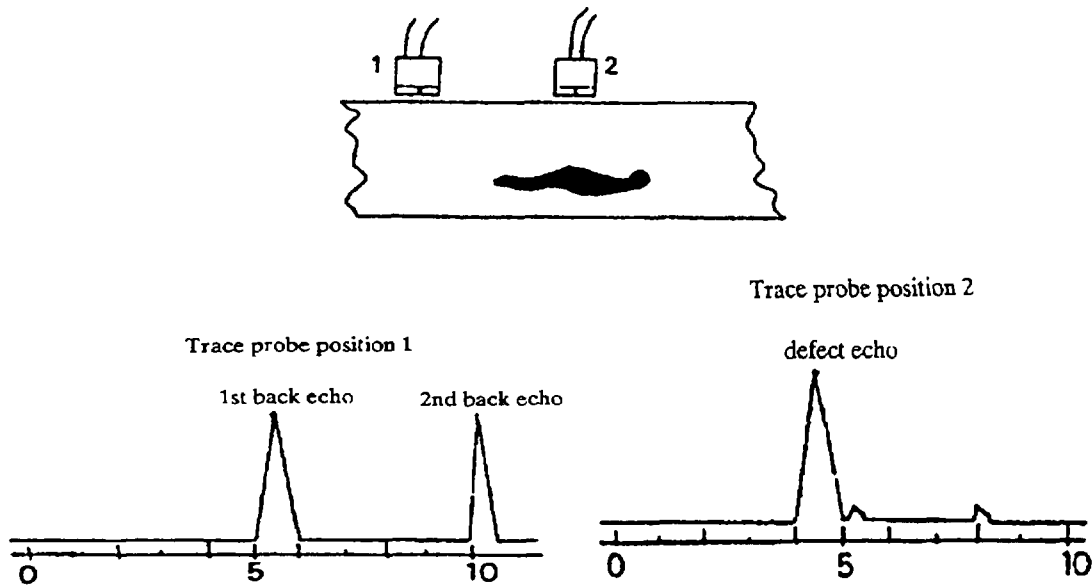
Figure 6.6 : Typical probe positions and resulting CRT screen appearance for testing of air locks.
