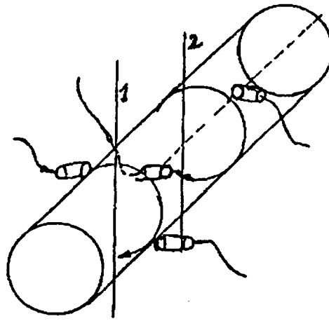
Figure 6.60 : Testing method for longitudinal surface defects on rod material by the immersion technique with two pairs of TR probes.
