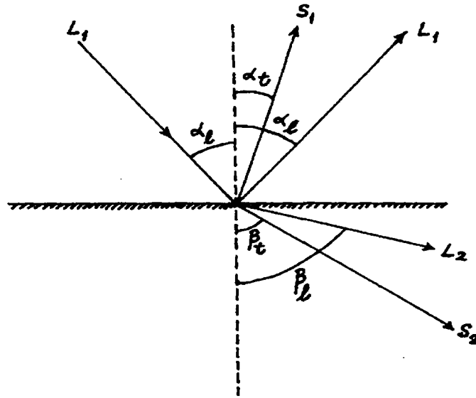
Figure 2.13 : Refraction and mode conversion for an incident longitudinal wave.
