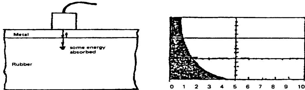
Figure 6.34 : Echo pattern indicating good bonded joint
