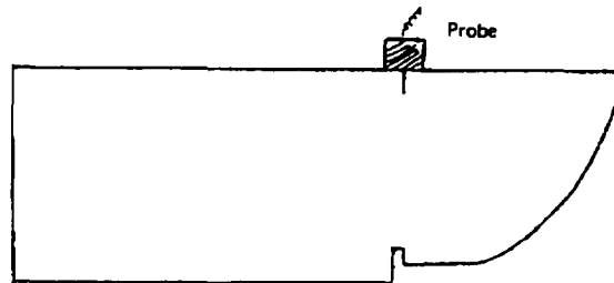
Figure 5.6 : (a) Placement of probe on I.I.W V1 block to determine the resolution of flaw detector and probe system.
