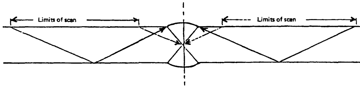
Figure 6.29 : Marking scan area for double-vee welds.
