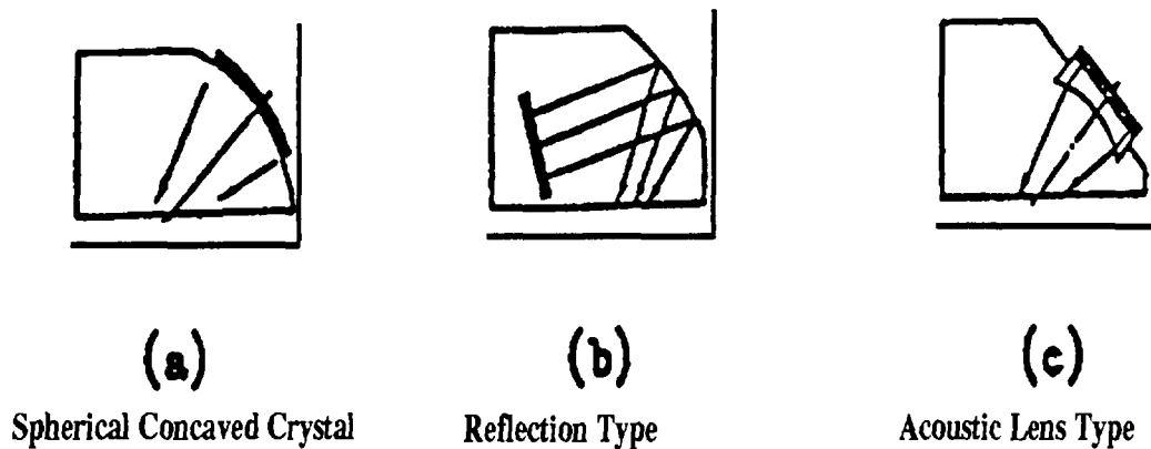
Figure 9.9 : Different ways of making focused probes.
