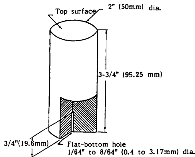
Figure 5.4 : Area-amplitude block.
