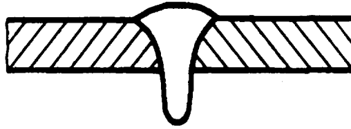
Figure 1.45 : Excessive penetration.
