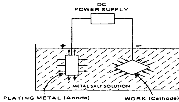
Figure 1.65 : Electroplating.
