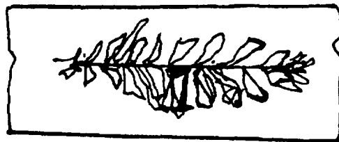
Figure 1.40 : Piping in weld.
