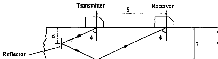
Figure 3.27 : Tandem technique arrangement.
